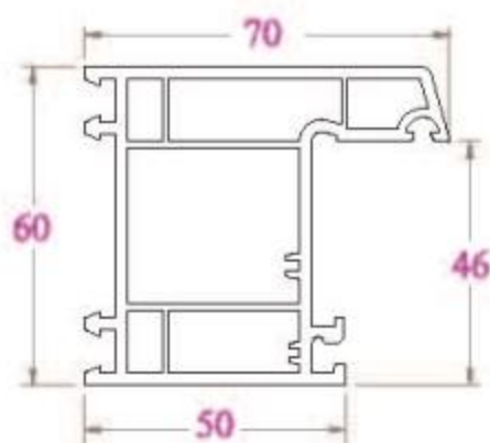
KHUÔN CỬA MK60 - 1154 g/m
