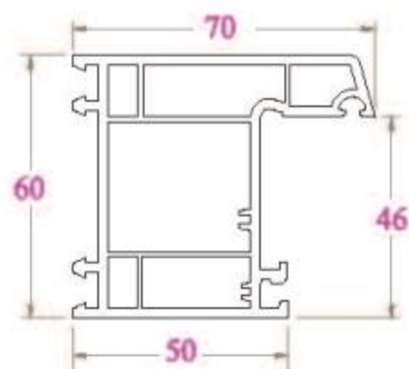
KHUÔN CỬA MK60 - 1154 g/m
