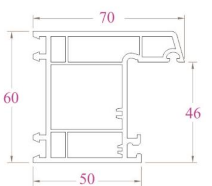
KHUÔN CỬA MK60 - 1154 g/m
