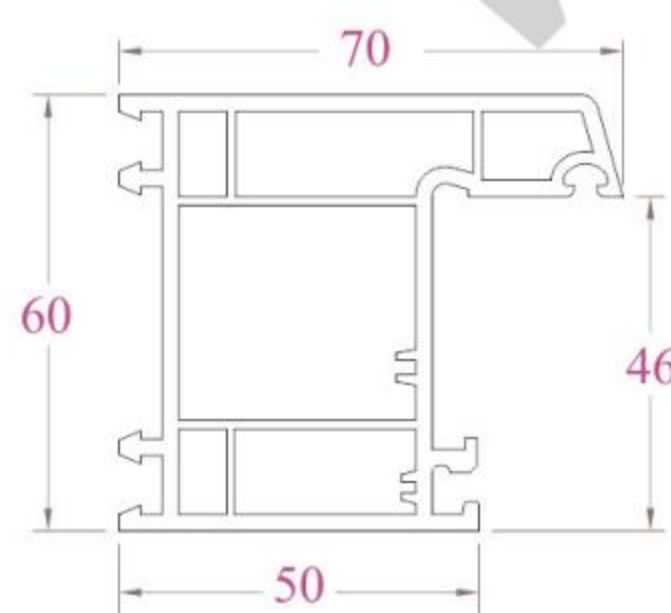
KHUÔN CỬA MK60 - 1154 g/m
