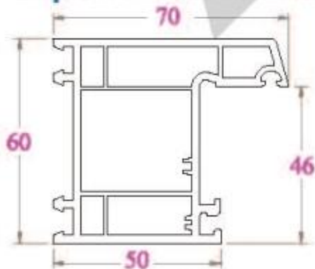
KHUÔN CỬA MK60 - 1154 g/m
