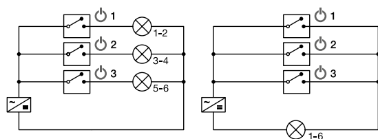
OR circuit
