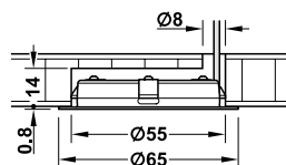
Recess mounting / Lắp âm
